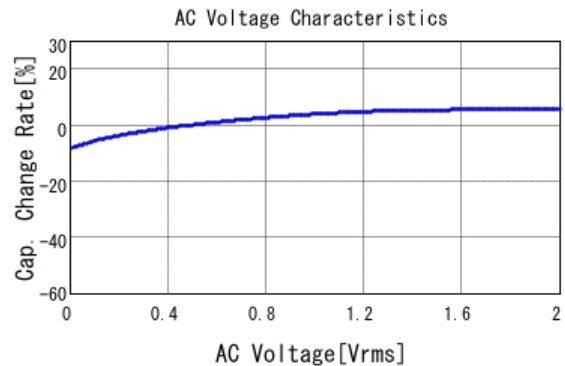
■ GRM155B31A474KE14 C-AC Voltage capchange, DCOV, 20.0d
