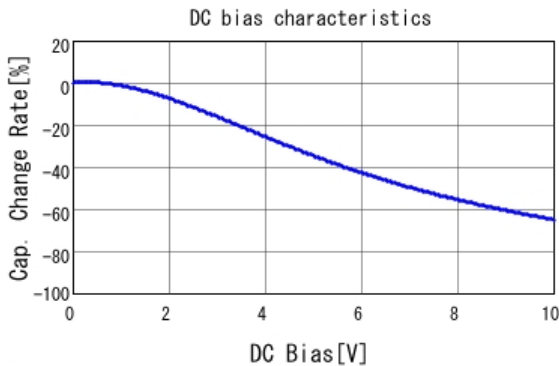
■ GRM155B31A474KE14 C-DC bias capchange, 20.0degC, AC0.
