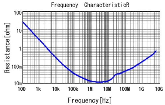
■ GRM155B31A474KE14 R DCOV, 20degC
