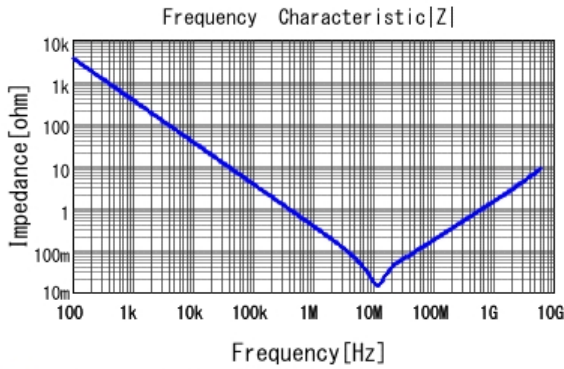
■ GRM155B31A474KE14 |Z| DCOV, 20degC
