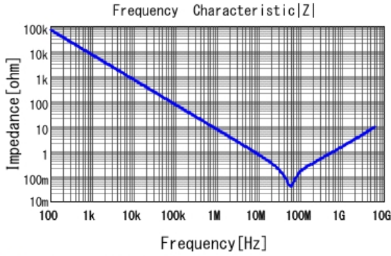
■ GRM155B31H223KA12 |Z| DCOV, 20degC
