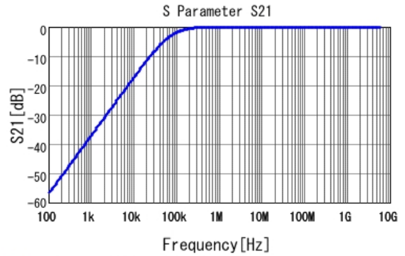
■ GRM155B31H223KA12 S21 DC0V, 20degC
