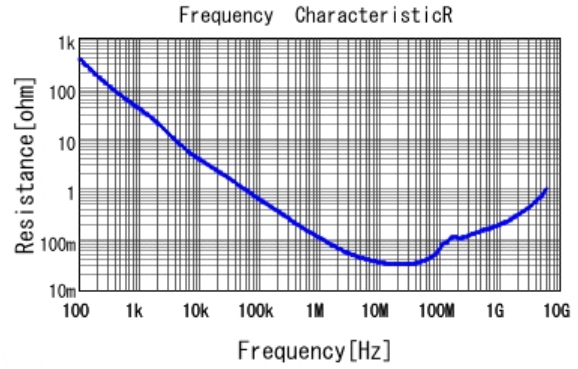
■ GRM155B31H223KA12 R DCOV, 20degC
