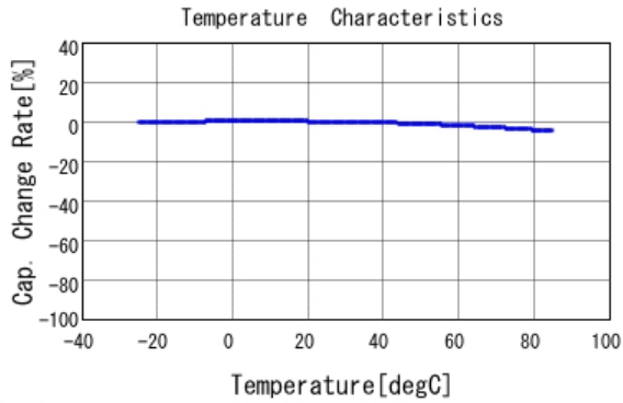
■ GRM155B31H223KA12 C-Temp. capchange, DC0.0V, AC1.0Vrm
