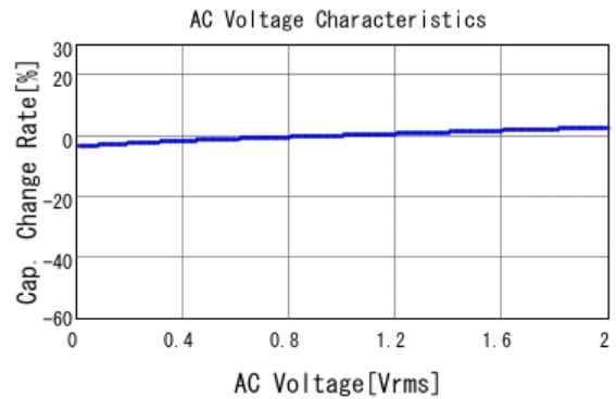
■ GRM155B31H223KA12 C-AC Voltage capchange, DCOV, 20.0d
