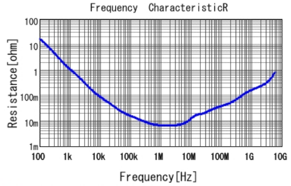
■ GRM155C80J225ME95 R DCOV, 25degC
