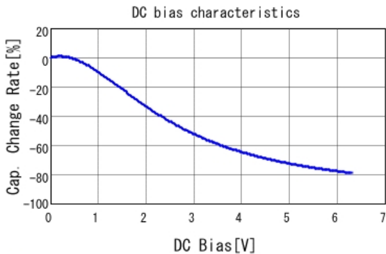
■ GRM155C80J225ME95 C-DC bias capchange, 25.0degC, ACO.
