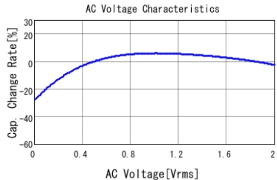
■ GRM155C80J225ME95 C-AC Voltage capchange, DCOV, 25.0d
