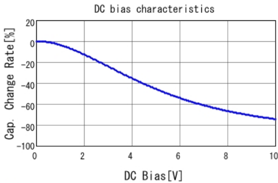
■ GRM155C81A225KE11 C-DC bias capchange, 25.0degC, AC1V
