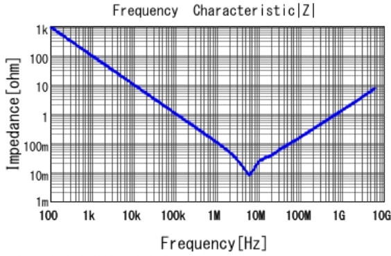
■ GRM155C81A225KE11 |Z| DCOV, 25degC
