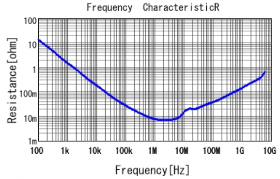
■ GRM155C81A225KE11 R DCOV, 25degC
