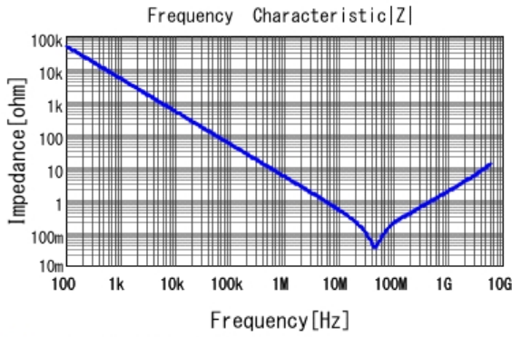
■ GRM155R11E333KA88 |Z| DCOV, 20degC
