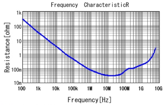
■ GRM155R11E333KA88 R DCOV, 20degC
