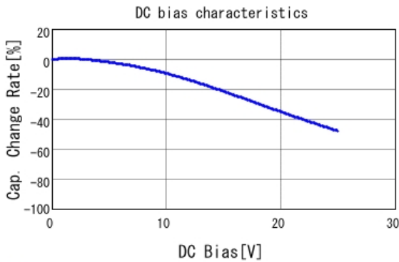
■ GRM155R11E333KA88 C-DC bias capchange, 20.0degC, AC1.
