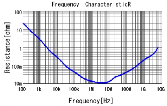
■ GRM155R60J105ME19 R DCOV, 25degC
