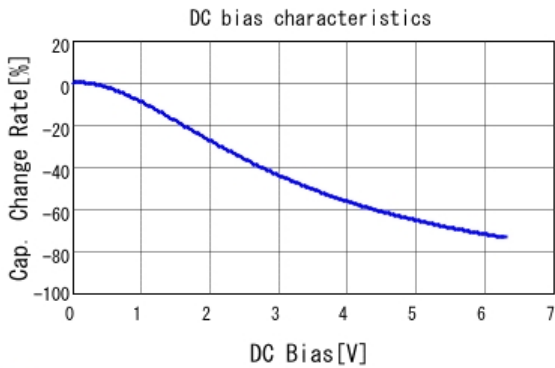
■ GRM155R60J105ME19 C-DC bias capchange, 25.0degC, AC0.
