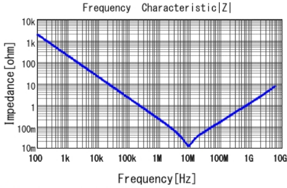
■ GRM155R60J105ME19 |Z| DCOV, 25degC
