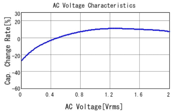
■ GRM155R60J105ME19 C-AC Voltage capchange, DCOV, 25.0d
