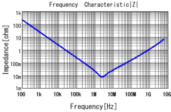
■ GRM155R60J106ME05 |Z| DCOV, 25degC
