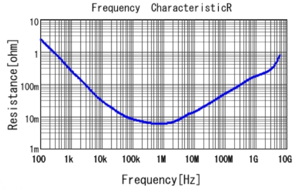
■ GRM155R60J106ME05 R DCOV, 25degC
