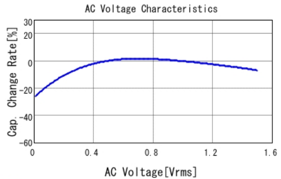
■ GRM155R60J106ME05 C-AC Voltage capchange, DCOV, 25.0d
