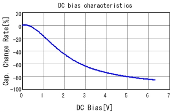
■ GRM155R60J106ME05 C-DC bias capchange, 25.0degC, AC0.
