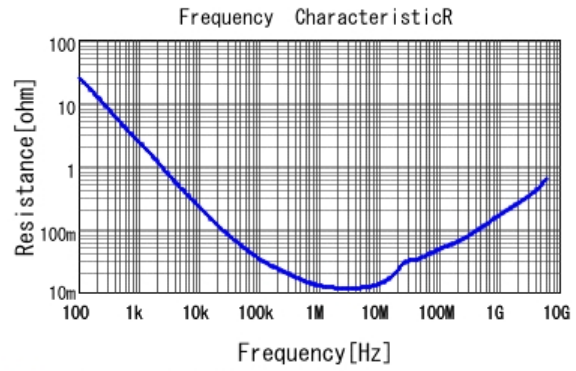
■ GRM155R60J474KE19 R DCOV, 25degC
