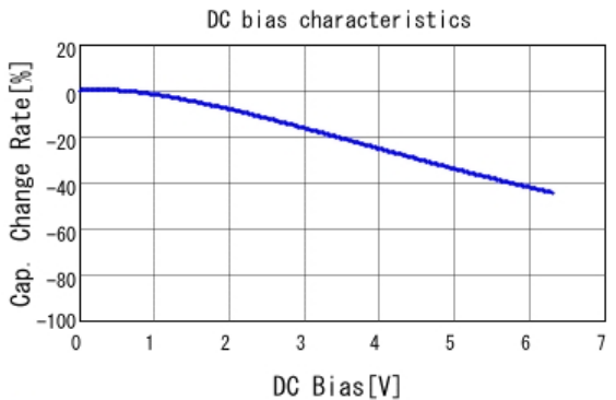
■ GRM155R60J474KE19 C-DC bias capchange, 25.0degC, AC0.
