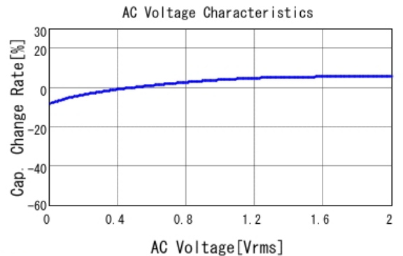
■ GRM155R60J474KE19 C-AC Voltage capchange, DCOV, 25.0d
