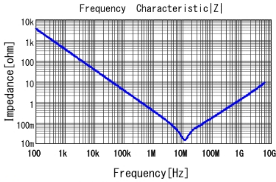
■ GRM155R60J474KE19 |Z| DCOV, 25degC
