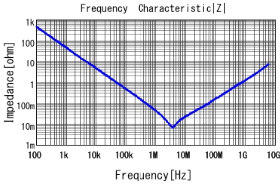
■ GRM155R60J475ME47 |Z| DCOV, 25degC
