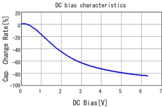
■ GRM155R60J475ME47 C-DC bias capchange, 25.0degC, ACO.
