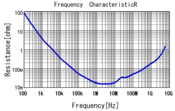
■ GRM155R61A105KE01 R DCOV, 25degC
