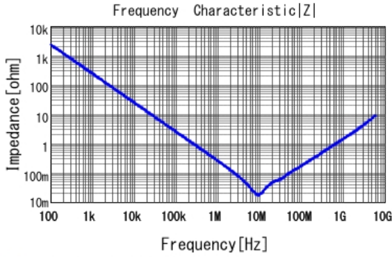
■ GRM155R61A105KE01 |Z| DCOV, 25degC
