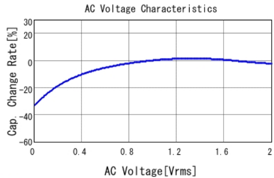
■ GRM155R61A105KE01 C-AC Voltage capchange, DCOV, 25.0d
