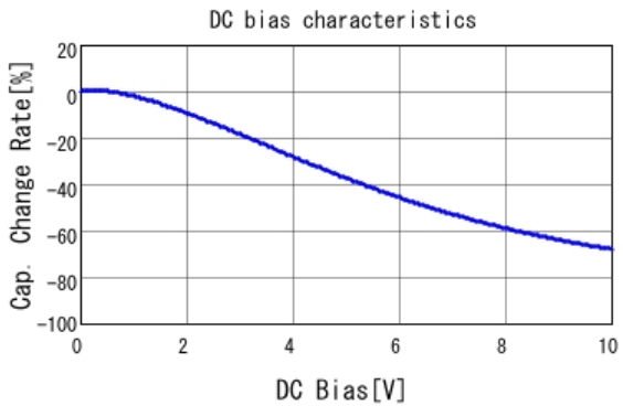
■ GRM155R61A105KE15 C-DC bias capchange, 25.0degC, AC0.
