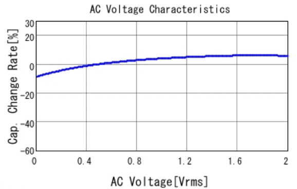
■ GRM155R61A105KE15 C-AC Voltage capchange, DCOV, 25.0d
