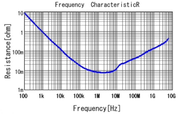
■ GRM155R61A105KE15 R DCOV, 25degC
