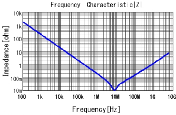
■ GRM155R61A105KE15 |Z| DCOV, 25degC
