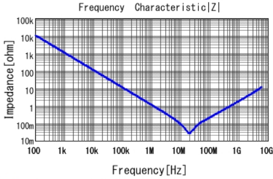
■ GRM155R61A154KE19 |Z| DCOV, 25degC
