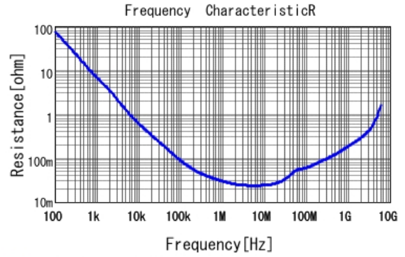
■ GRM155R61A154KE19 R DCOV, 25degC
