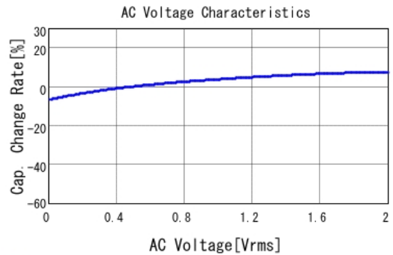
■ GRM155R61A154KE19 C-AC Voltage capchange, DCOV, 25.0d
