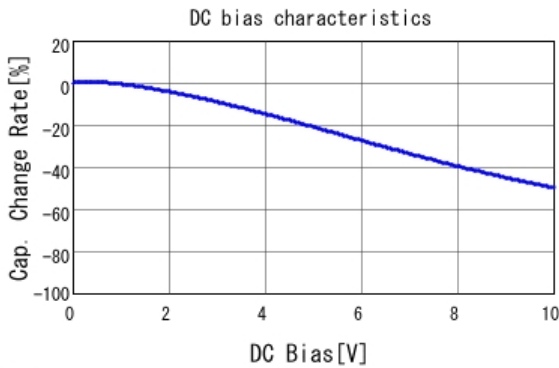
■ GRM155R61A154KE19 C-DC bias capchange, 25.0degC, AC0.
