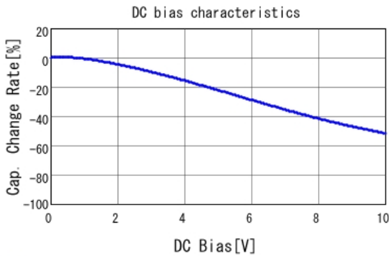
■ GRM155R61A224KE19 C-DC bias capchange, 25.0degC, AC0.
