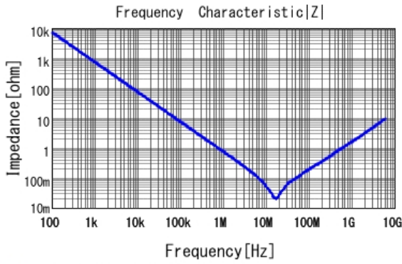
■ GRM155R61A224KE19 |Z| DCOV, 25degC
