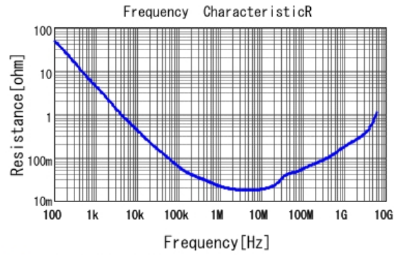
■ GRM155R61A224KE19 R DCOV, 25degC
