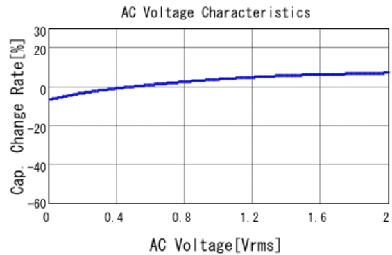
■ GRM155R61A224KE19 C-AC Voltage capchange, DCOV, 25.0d
