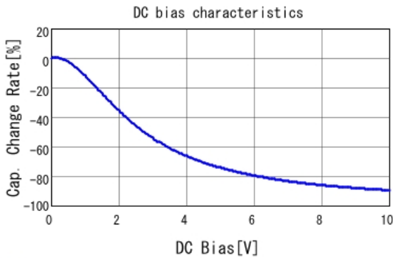
■ GRM155R61A225ME01 C-DC bias capchange, 25.0degC, AC0.
