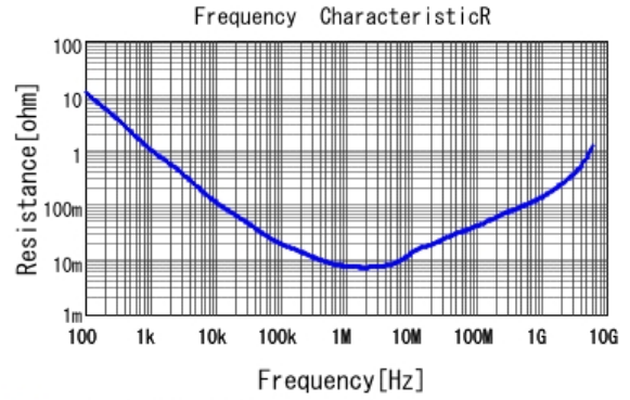
■ GRM155R61A225ME01 R DCOV, 25degC
