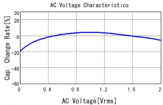
■ GRM155R61A225ME01 C-AC Voltage capchange, DCOV, 25.0d
