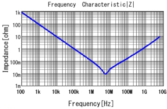
■ GRM155R61A225ME01 |Z| DCOV, 25degC
