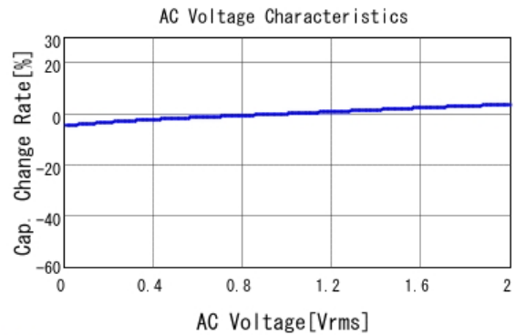
■ GRM155R61A333KA01 C-AC Voltage capchange, DCOV, 25.0d
