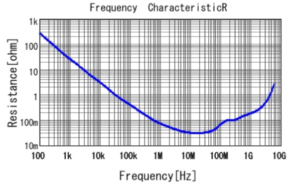
■ GRM155R61A333KA01 R DCOV, 25degC
