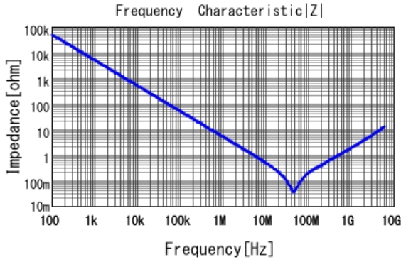
■ GRM155R61A333KA01 |Z| DCOV, 25degC
