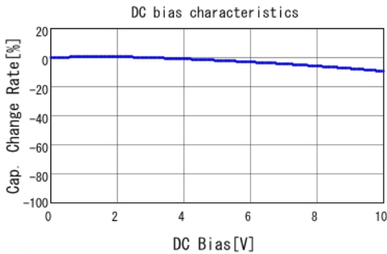
■ GRM155R61A333KA01 C-DC bias capchange, 25.0degC, AC1.
