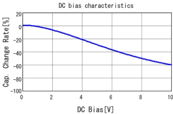
■ GRM155R61A334KE15 C-DC bias capchange, 25.0degC, AC0.
