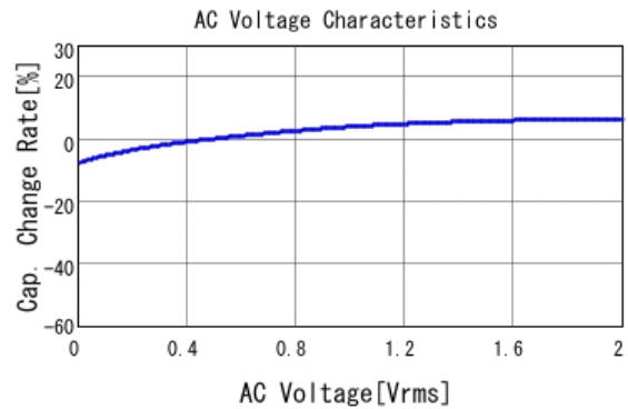
■ GRM155R61A334KE15 C-AC Voltage capchange, DCOV, 25.0d
