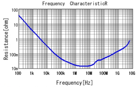
■ GRM155R61A334KE15 R DCOV, 25degC
