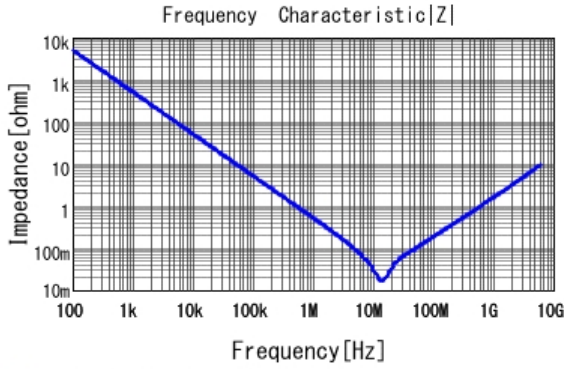
■ GRM155R61A334KE15 |Z| DCOV, 25degC
