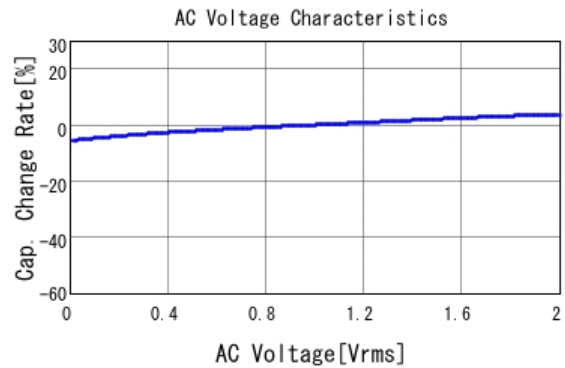
■ GRM155R61A473KA01 C-AC Voltage capchange, DCOV, 25.0d
