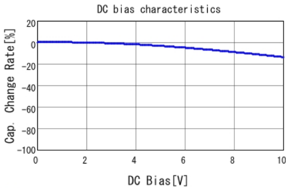
■ GRM155R61A473KA01 C-DC bias capchange, 25.0degC, AC1.
