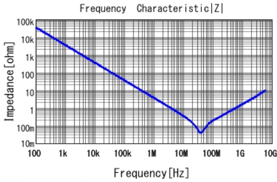
■ GRM155R61A473KA01 |Z| DCOV, 25degC
