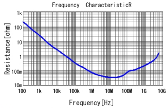
■ GRM155R61A473KA01 R DCOV, 25degC
