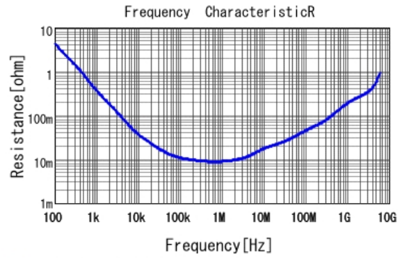
■ GRM155R61A475MEAA R DCOV, 25degC
