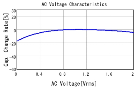
■ GRM155R61A475MEAA C-AC Voltage capchange, DCOV, 25.0d
