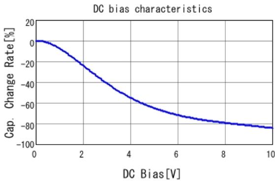
■ GRM155R61A475MEAA C-DC bias capchange, 25.0degC, AC1V
