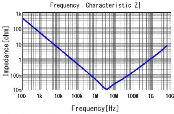
■ GRM155R61A475MEAA |Z| DCOV, 25degC
