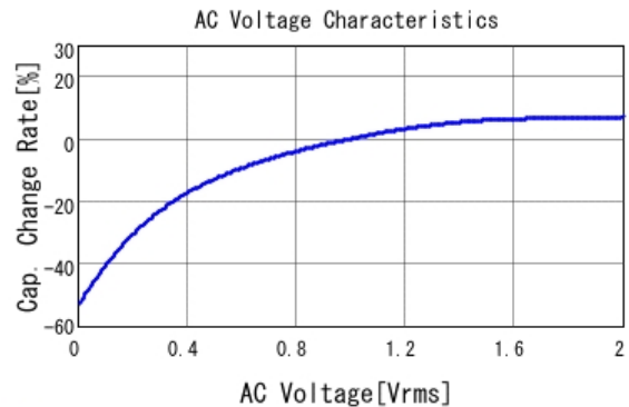
■ GRM155R61C105KA12 C-AC Voltage capchange, DCOV, 25.0d
