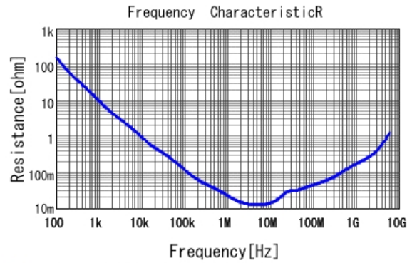
■ GRM155R61C105KA12 R DCOV, 25degC
