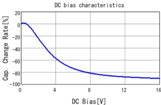
■ GRM155R61C105KA12 C-DC bias capchange, 25.0degC, AC1.
