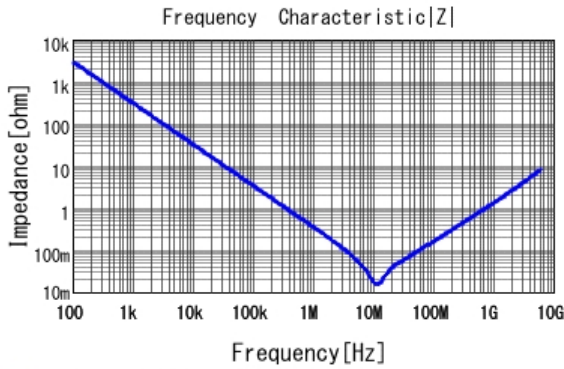
■ GRM155R61C105KA12 |Z| DCOV, 25degC
