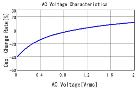
■ GRM155R61C224KA12 C-AC Voltage capchange, DCOV, 25.0d
