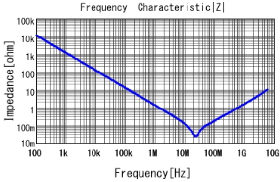
■ GRM155R61C224KA12 |Z| DCOV, 25degC
