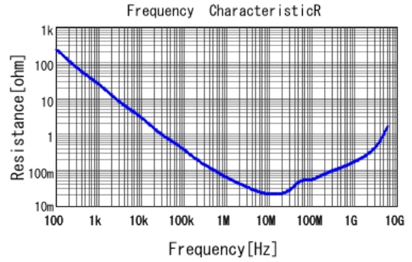
■ GRM155R61C224KA12 R DCOV, 25degC
