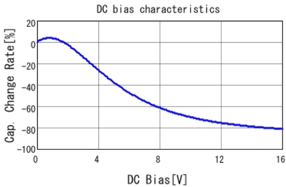
■ GRM155R61C224KA12 C-DC bias capchange, 25.0degC, AC1.
