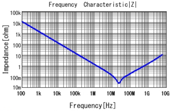
■ GRM155R61C224MA12 |Z| DCOV, 25degC
