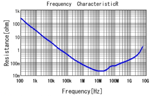
■ GRM155R61C224MA12 R DCOV, 25degC
