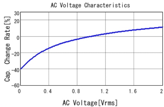
■ GRM155R61C224MA12 C-AC Voltage capchange, DCOV, 25.0d
