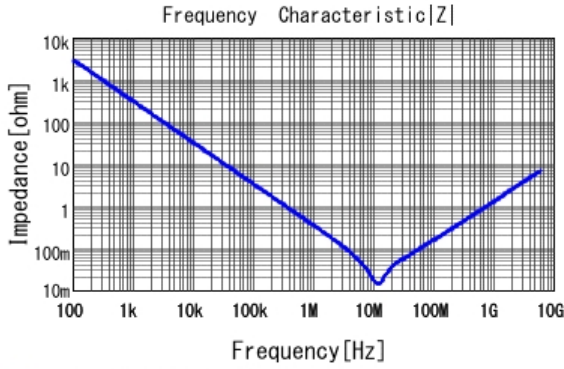
■ GRM155R61E105KA12 |Z| DCOV, 25degC
