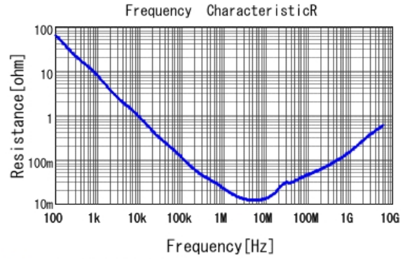
■ GRM155R61E105KA12 R DCOV, 25degC
