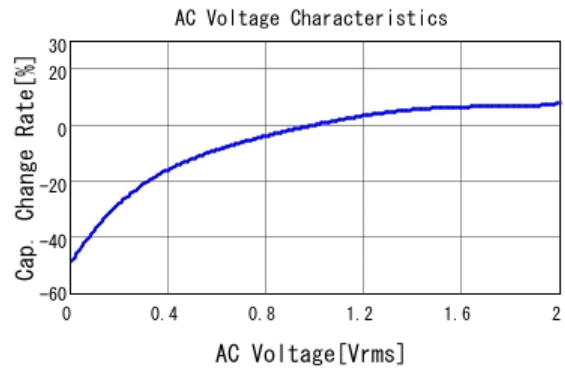
■ GRM155R61E105KA12 C-AC Voltage capchange, DCOV, 25.0d
