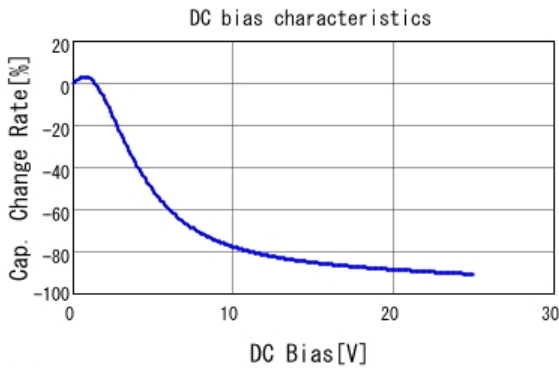
■ GRM155R61E474KE01 C-DC bias capchange, 25.0degC, AC1.
