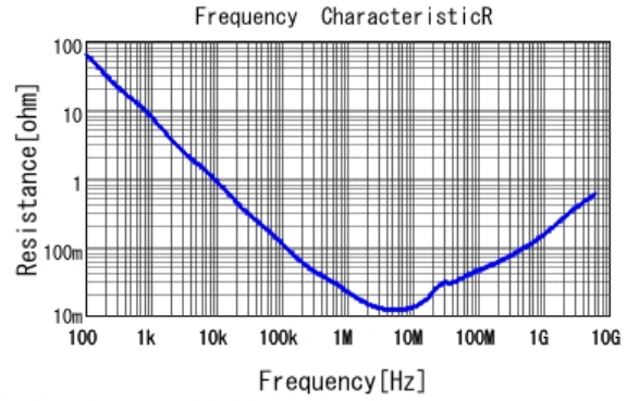
■ GRM155R70J105KA12 R DCOV, 25degC
