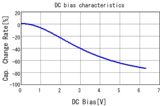
■ GRM155R70J105KA12 C-DC bias capchange, 25.0degC, AC1V
