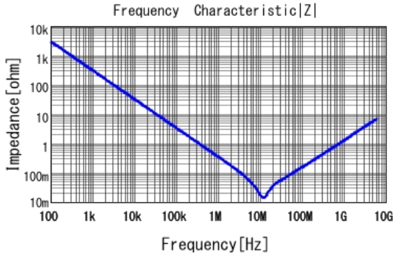
■ GRM155R70J105KA12 |Z| DCOV, 25degC
