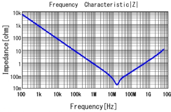
■ GRM155R71A474KE01 |Z| DC0V, 25degC
