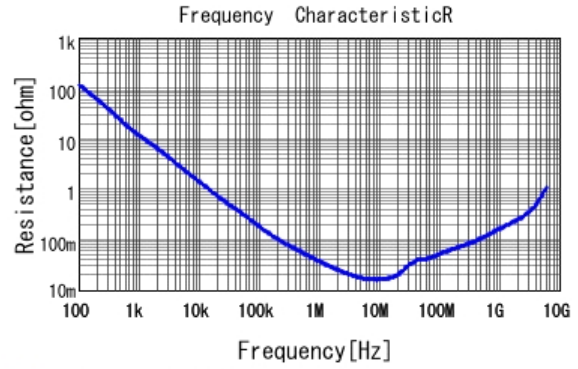
■ GRM155R71A474KE01 R DC0V, 25degC
