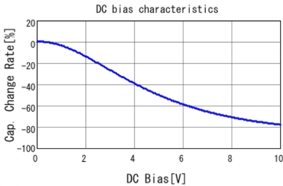
■ GRM155R71A474KE01 C-DC bias capchange, 25.0degC, AC1V
