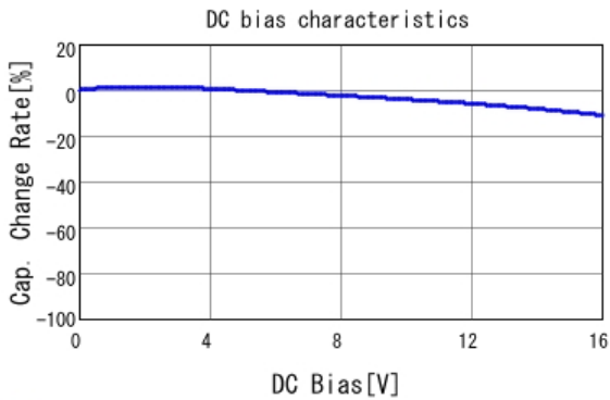
■ GRM155R71C103KA01 C-DC bias capchange, 25.0degC, AC1.
