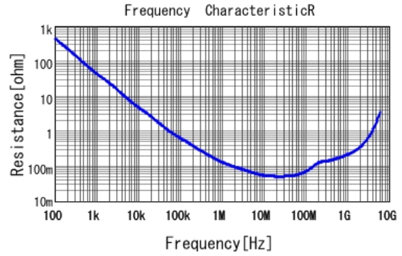
■ GRM155R71C183KA01 R DCOV, 25degC
