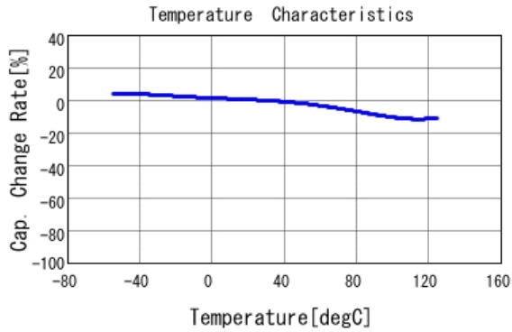
■ GRM155R71C183KA01 C-Temp. capchange, DC0.0V, AC1.0V rm
