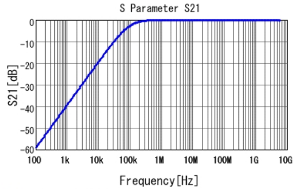
■ GRM155R71C183KA01 S21 DC0V, 25degC
