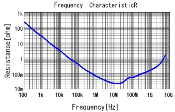
■ GRM155R71C224KA12 R DCOV, 25degC
