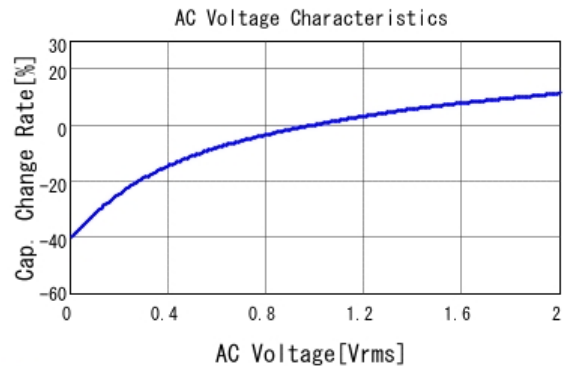
■ GRM155R71C224KA12 C-AC Voltage capchange, DCOV, 25.0d
