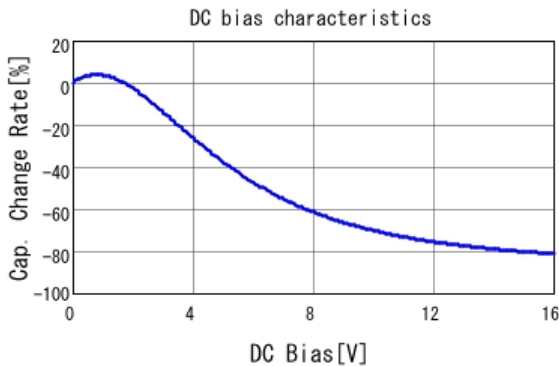
■ GRM155R71C224KA12 C-DC bias capchange, 25.0degC, AC1.
