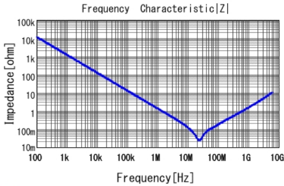
■ GRM155R71C224KA12 |Z| DCOV, 25degC
