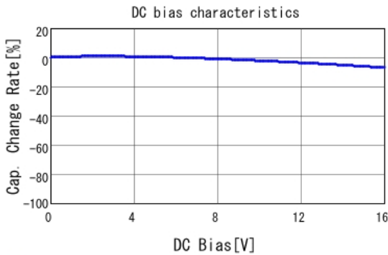
■ GRM155R71C472KA01 C-DC bias capchange, 25.0degC, AC1.
