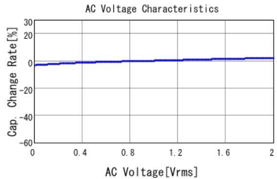
■ GRM155R71C472KA01 C-AC Voltage capchange, DCOV, 25.0d
