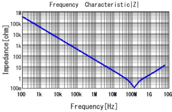
■ GRM155R71C472KA01 |Z| DCOV, 25degC
