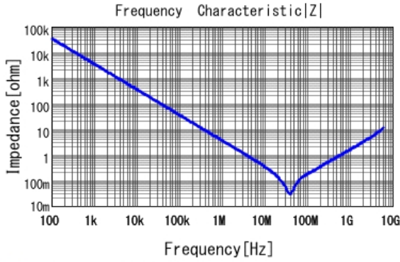
■ GRM155R71C473KA01 |Z| DCOV, 25degC
