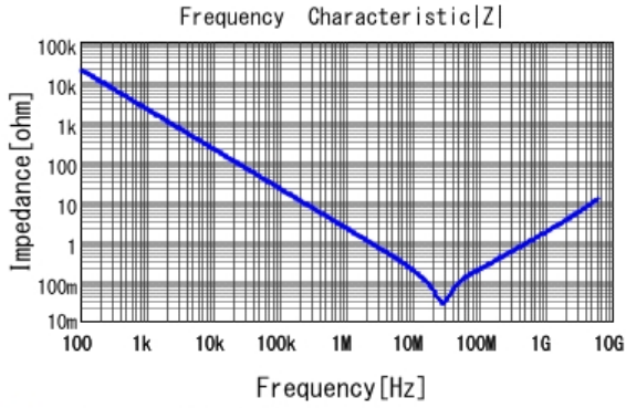
■ GRM155R71C823KA88 |Z| DCOV, 25degC
