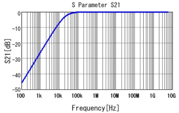
■ GRM155R71C823KA88 S21 DC0V, 25degC
