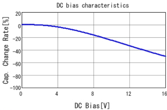
■ GRM155R71C823KA88 C-DC bias capchange, 25.0degC, AC1.
