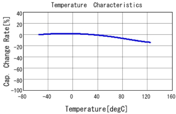
■ GRM155R71C823KA88 C-Temp. capchange, DC0.0V, AC1.0V rm
