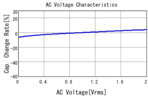
■ GRM155R71C823KA88 C-AC Voltage capchange, DCOV, 25.0d
