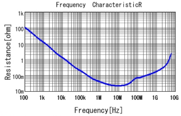
■ GRM155R71C823KA88 R DCOV, 25degC
