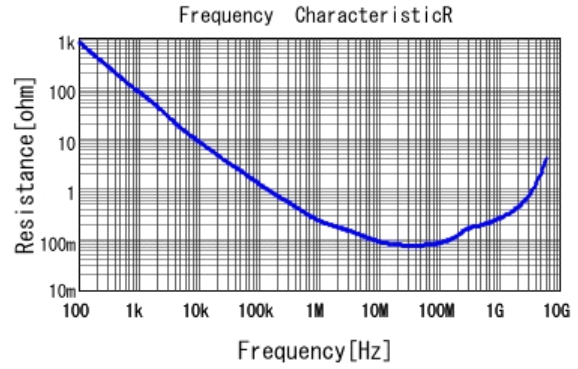
■ GRM155R71E103KA01 R DCOV, 25degC
