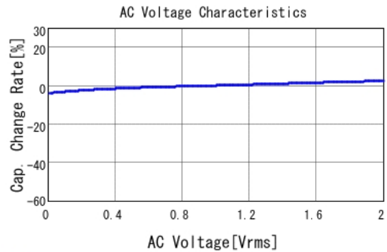
■ GRM155R71E103KA01 C-AC Voltage capchange, DCOV, 25.0d
