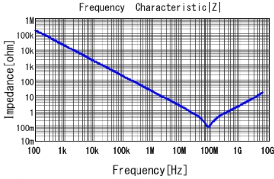
■ GRM155R71E103KA01 |Z| DCOV, 25degC
