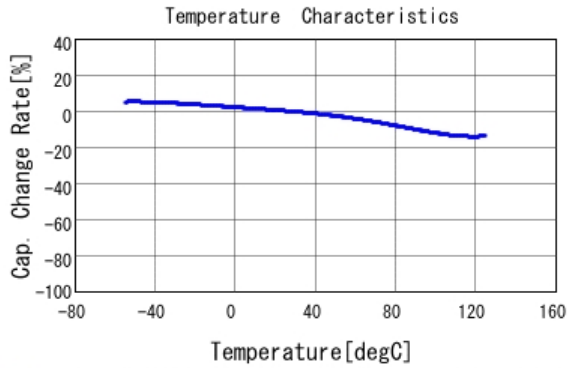
■ GRM155R71E223KA61 C-Temp. capchange, DC0.0V, AC1.0Vrm
