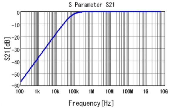
■ GRM155R71E223KA61 S21 DC0V, 25degC
