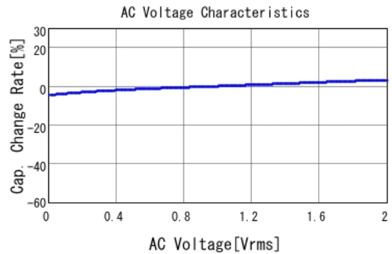
■ GRM155R71E473KA88 C-AC Voltage capchange, DCOV, 25.0d
