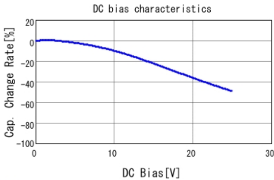
■ GRM155R71E473KA88 C-DC bias capchange, 25.0degC, AC1.
