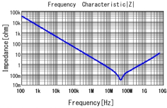
■ GRM155R71E473KA88 |Z| DCOV, 25degC
