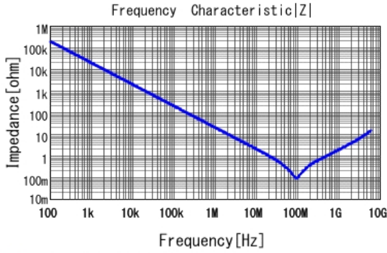
■ GRM155R71E822KA01 |Z| DCOV, 25degC
