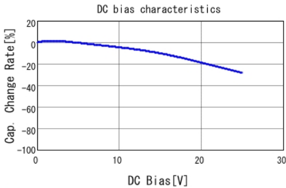
■ GRM155R71E822KA01 C-DC bias capchange, 25.0degC, AC1.
