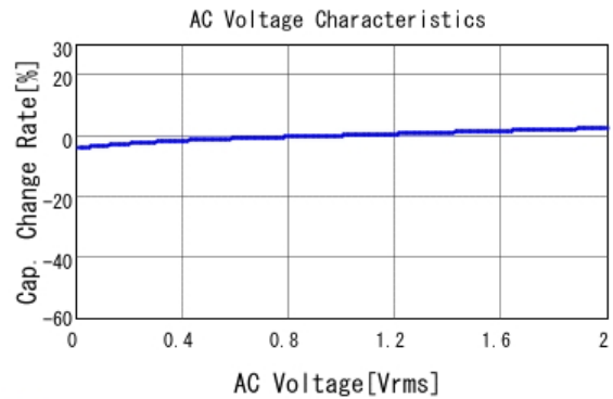
■ GRM155R71E822KA01 C-AC Voltage capchange, DCOV, 25.0d
