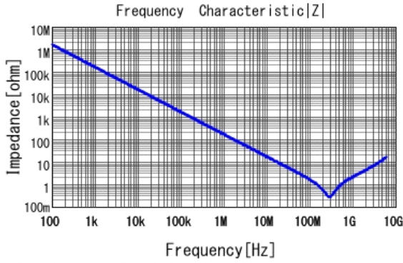
■ GRM155R71H102KA01 |Z| DCOV, 25degC
