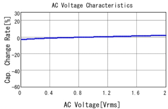
■ GRM155R71H102KA01 C-AC Voltage capchange, DCOV, 25.0d
