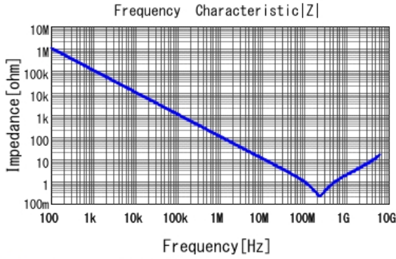
■ GRM155R71H152KA01 |Z| DCOV, 25degC
