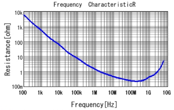
■ GRM155R71H152KA01 R DCOV, 25degC
