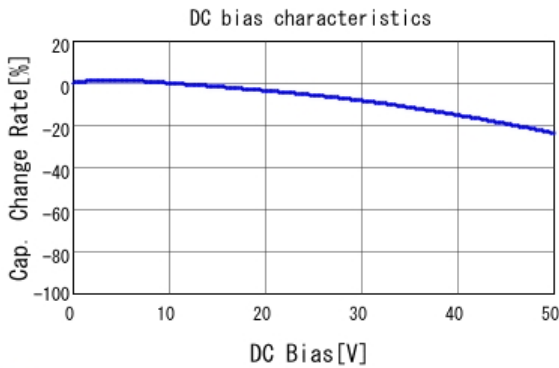
■ GRM155R71H221KA01 C-DC bias capchange, 25.0degC, AC1.
