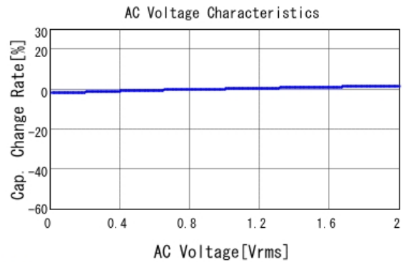
■ GRM155R71H221KA01 C-AC Voltage capchange, DCOV, 25.0d
