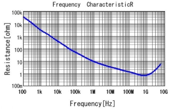
■ GRM155R71H221KA01 R DCOV, 25degC
