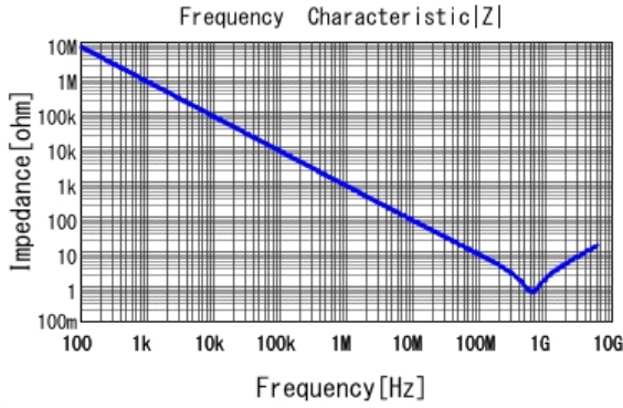
■ GRM155R71H221KA01 |Z| DCOV, 25degC
