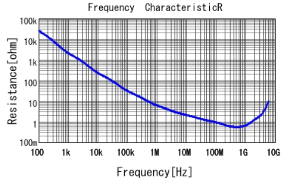
■ GRM155R71H331KA01 R DCOV, 25degC
