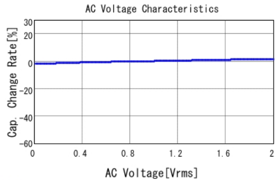
■ GRM155R71H331KA01 C-AC Voltage capchange, DCOV, 25.0d
