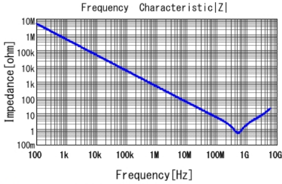
■ GRM155R71H331KA01 |Z| DCOV, 25degC
