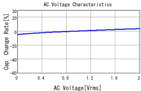
■ GRM155R71H333KE14 C-AC Voltage capchange, DCOV, 25.0d
