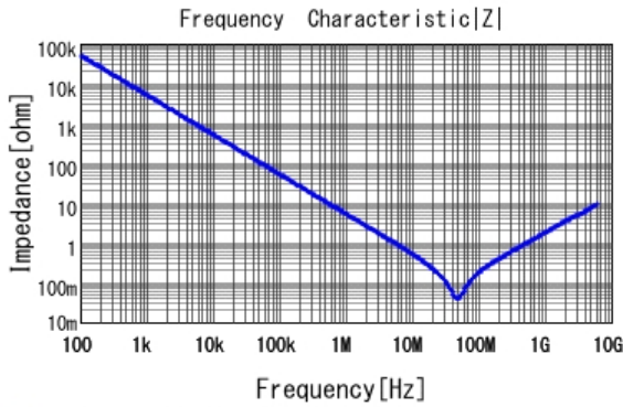
■ GRM155R71H333KE14 |Z| DCOV, 25degC
