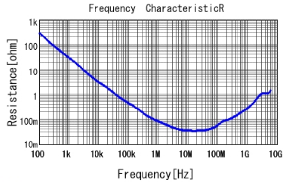
■ GRM155R71H333KE14 R DCOV, 25degC
