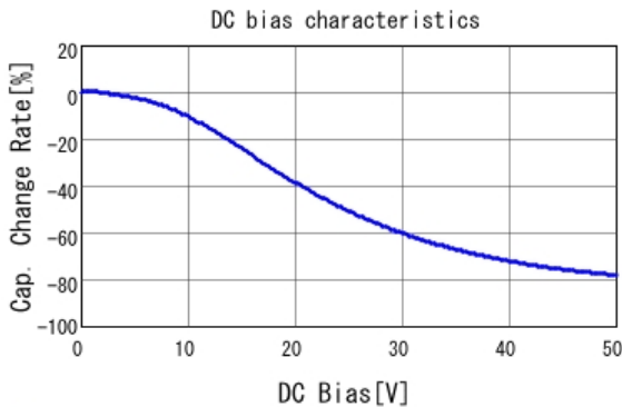
■ GRM155R71H333KE14 C-DC bias capchange, 25.0degC, AC1.
