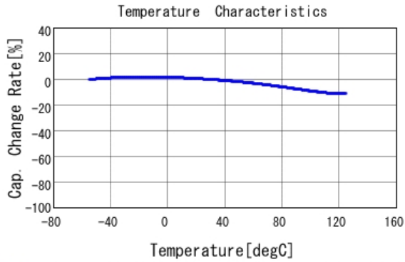
■ GRM155R71H333KE14 C-Temp. capchange, DC0.0V, AC1.0Vrm
