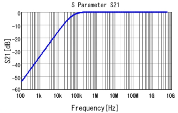
■ GRM155R71H333KE14 S21 DC0V, 25degC
