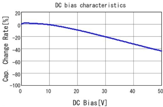
■ GRM155R71H392KA01 C-DC bias capchange, 25.0degC, AC1.
