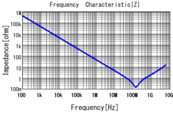
■ GRM155R71H392KA01 |Z| DCOV, 25degC
