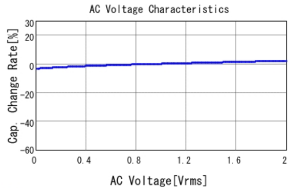
■ GRM155R71H392KA01 C-AC Voltage capchange, DCOV, 25.0d
