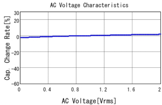
■ GRM155R71H561KA01 C-AC Voltage capchange, DCOV, 25.0d
