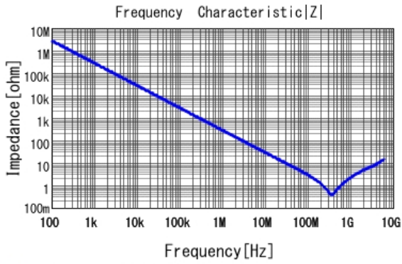
■ GRM155R71H561KA01 |Z| DCOV, 25degC
