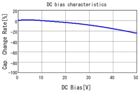
■ GRM155R71H561KA01 C-DC bias capchange, 25.0degC, AC1.
