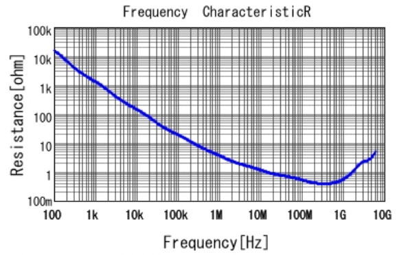
■ GRM155R71H561KA01 R DCOV, 25degC
