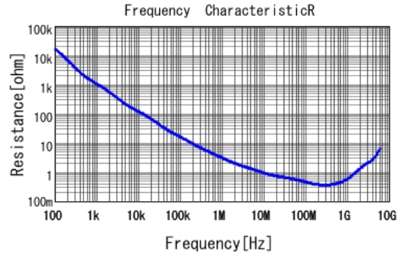
■ GRM155R71H681KA01 R DCOV, 25degC
