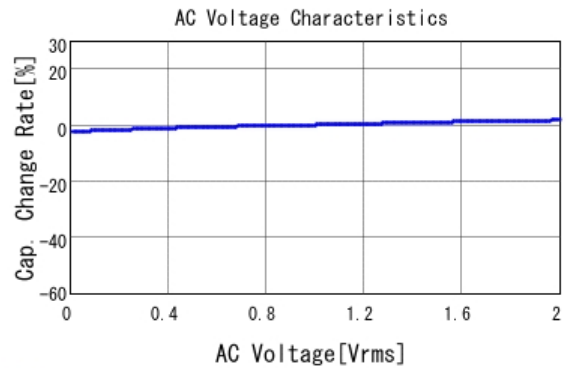
■ GRM155R71H681KA01 C-AC Voltage capchange, DCOV, 25.0d
