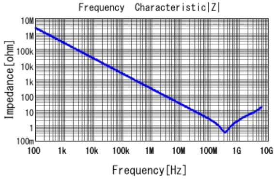
■ GRM155R71H681KA01 |Z| DCOV, 25degC
