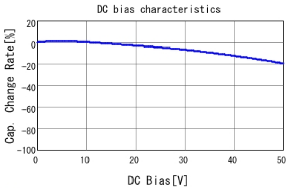
■ GRM155R71H681KA01 C-DC bias capchange, 25.0degC, AC1.
