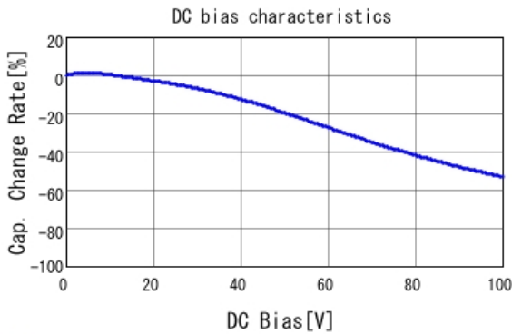
■ GRM155R72A681KA01 C-DC bias capchange, 25.0degC, AC1.
