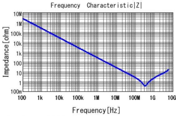
■ GRM155R72A681KA01 |Z| DCOV, 25degC
