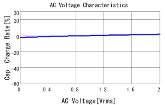
■ GRM155R72A681KA01 C-AC Voltage capchange, DCOV, 25.0d
