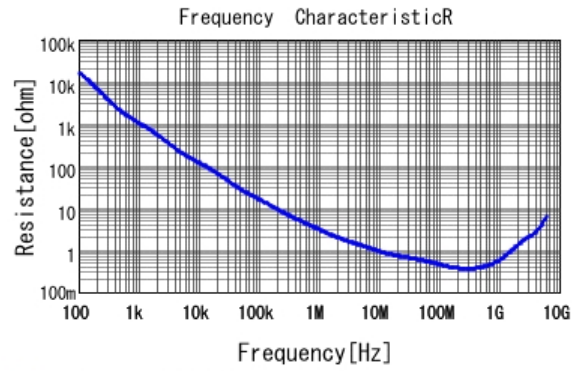
■ GRM155R72A681KA01 R DCOV, 25degC
