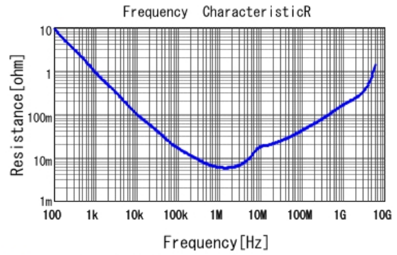
■ GRM185R61A475KE11 R DCOV, 25degC
