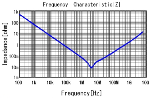
■ GRM185R61A475KE11 |Z| DCOV, 25degC
