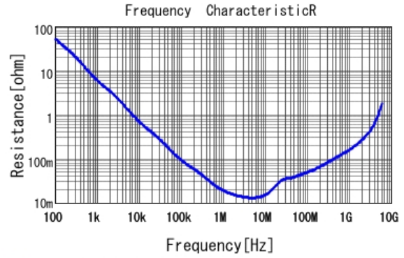
■ GRM185R61C105KE44 R DCOV, 25degC
