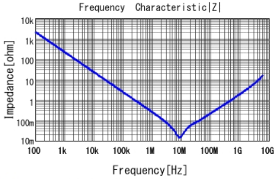
■ GRM185R61C105KE44 |Z| DCOV, 25degC
