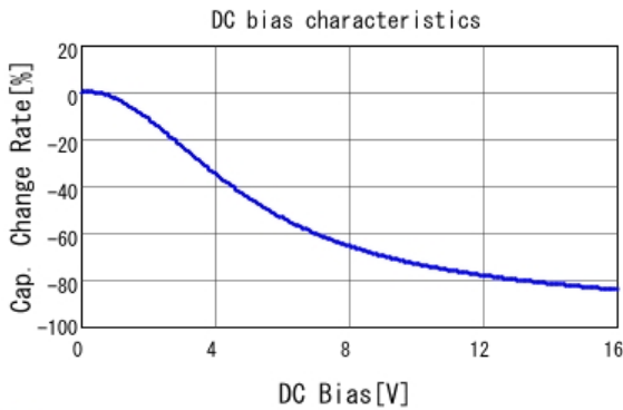
■ GRM185R61C105KE44 C-DC bias capchange, 25.0degC, AC0.
