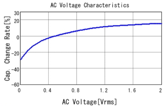
■ GRM185R61C105KE44 C-AC Voltage capchange, DCOV, 25.0d
