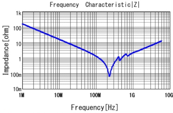
■ GRM1882C1E102JA01 |Z| DCOV, 20degC
