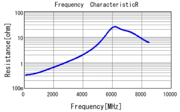
■ GRM1882C1H100JA01 R DCOV, 20degC
