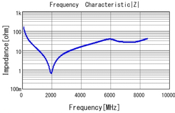
■ GRM1882C1H100JA01 |Z| DCOV, 20degC
