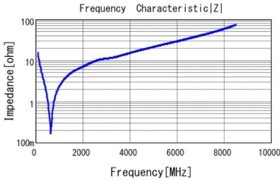
■ GRM1882C1H101JA01 |Z| DCOV, 20degC
