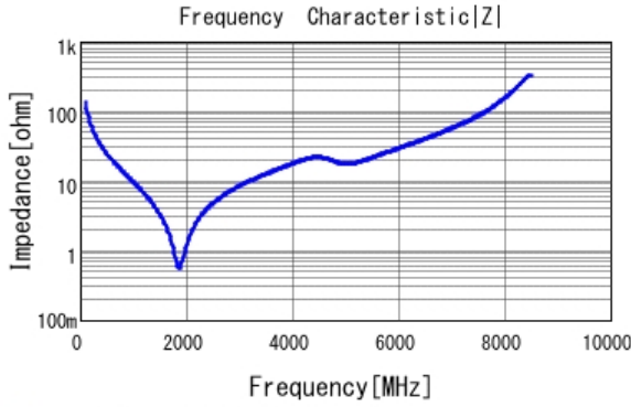
■ GRM1882C1H120JA01 |Z| DCOV, 20degC
