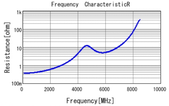
■ GRM1882C1H120JA01 R DCOV, 20degC
